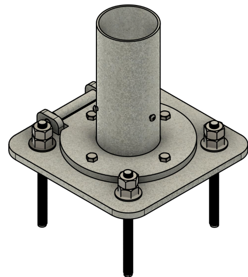
Hinged Base Detail
