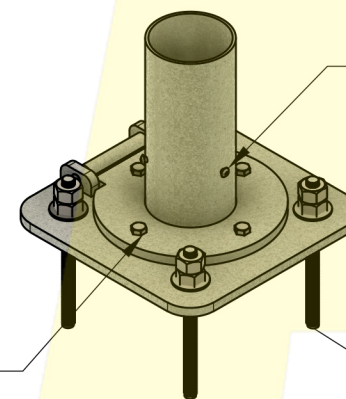
Base Connection Detail
