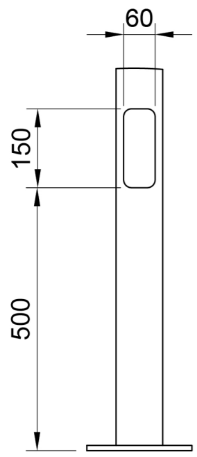
Cover Detail
